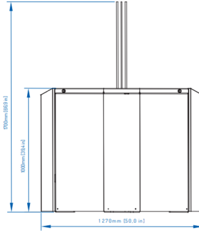
WIDE LANE FULL HEIGHT GLASS
