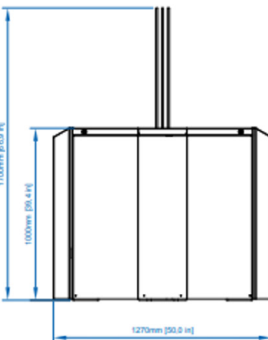
DDA LANE FULL HEIGHT GLASS
