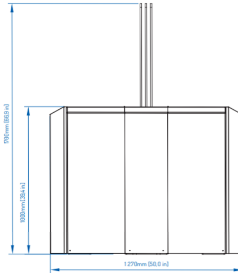
STANDARD LANE FULL HEIGHT GLASS
